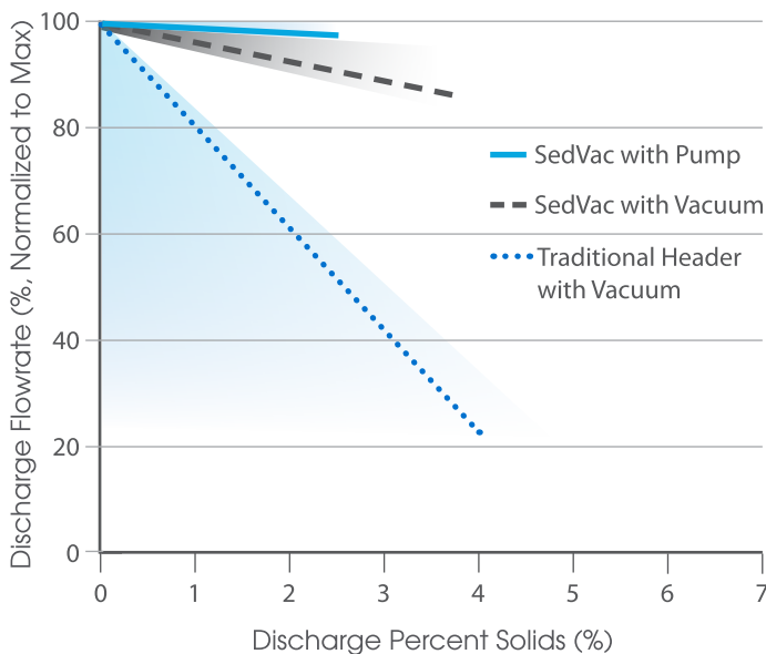
Figure 1: Discharge Flow Rate vs. Solids Concentration
