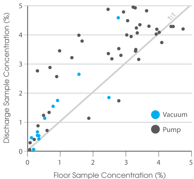
Figure 2: SedVac Sludge Concentrating Effect
